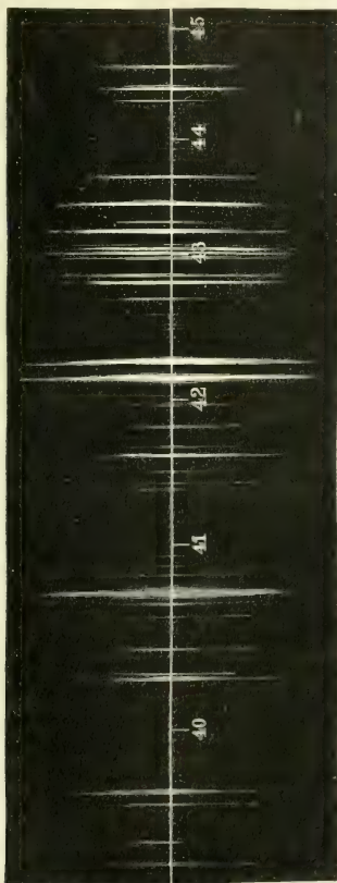
FIG. 17.—The long and short lines. Copy of a photograph taken with a vertical slit when the compounds of strontium and calcium were volatilised between horizontal carbon poles.
